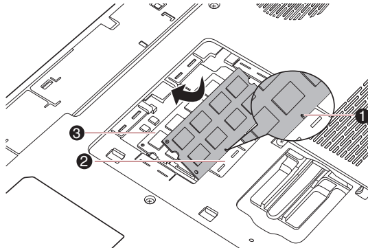
Figure 3-5 Seating the memory module
