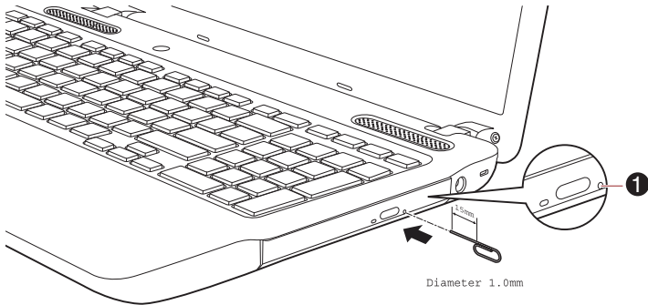
Figure 4-5 Manual release with the eject hole
