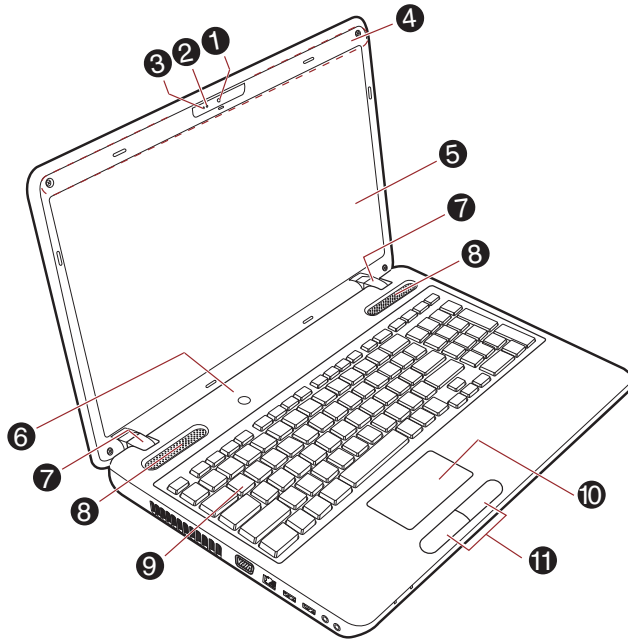
Figure 2-6 The front of the computer with the display panel open
