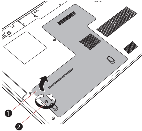
Figure 3-4 Removing the memory module cover
