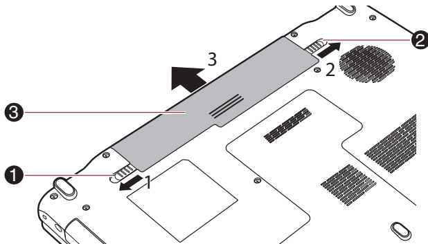
Figure 6-1 Releasing the battery pack
