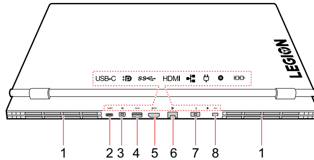
Figure 7. Lenovo Legion Y540-15 and Legion Y540-15 series - rear view
