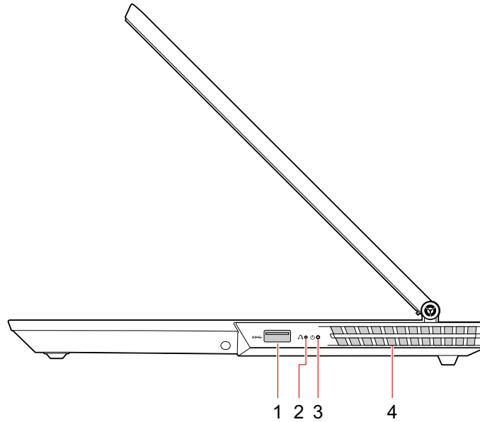
Figure 5. Lenovo Legion Y540-15 and Legion Y540-15 series - right view
