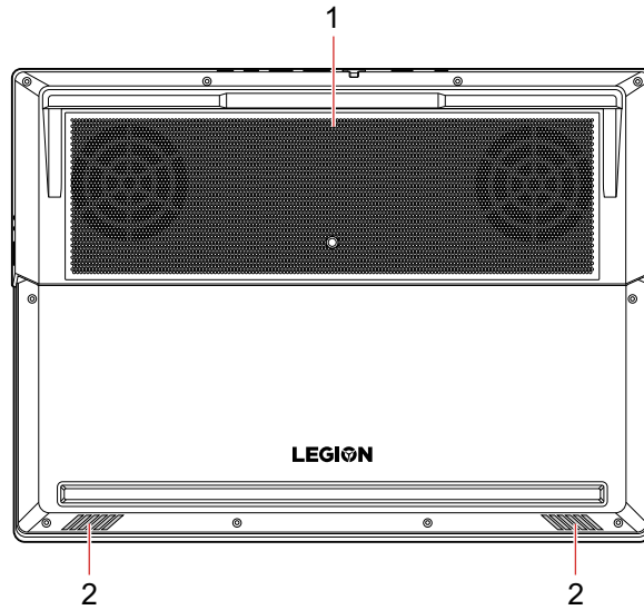
Figure 9. Lenovo Legion Y540-15 and Legion Y540-15 series - bottom view
