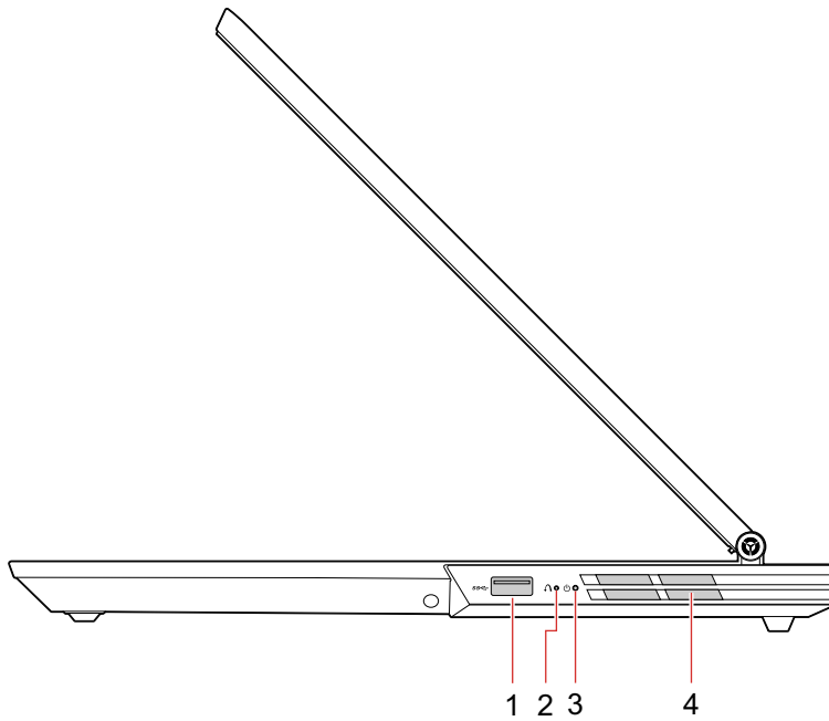
Figure 6. Lenovo Legion Y540-17 and Legion Y540-17 series - right view
