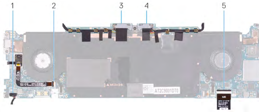
Figure 1. System-board connectors
