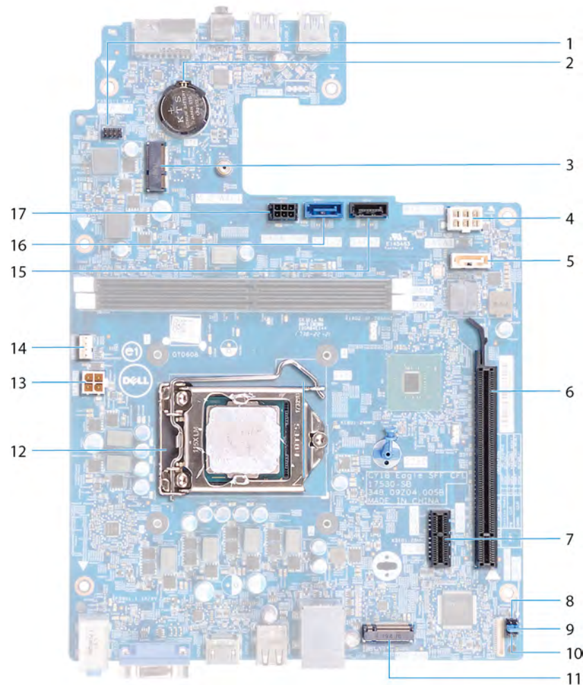
Figure 2. System-board components
