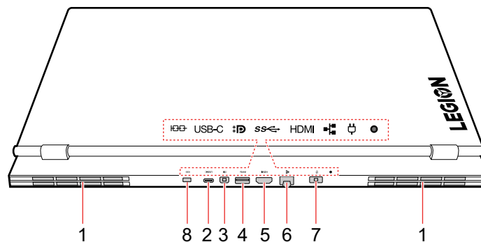
Figure 8. Legion Y540-17 series - rear view
