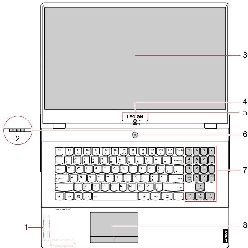
Figure 2. Legion Y540-17 series - front view
