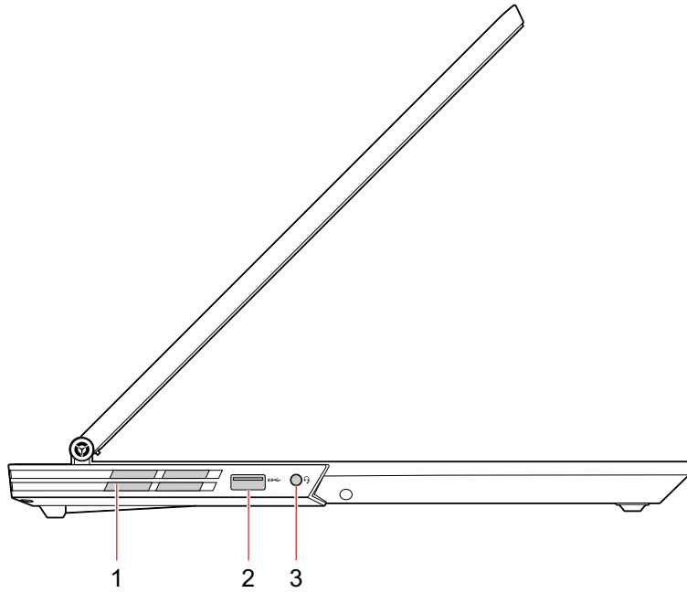
Figure 4. Legion Y540-17 series - left view
