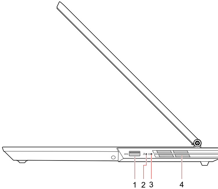
Figure 6. Legion Y540-17 series - right view
