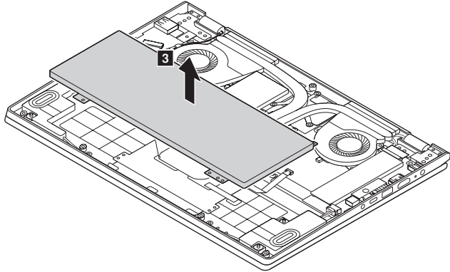
Figure 2. Removal steps of battery pack (continued)
