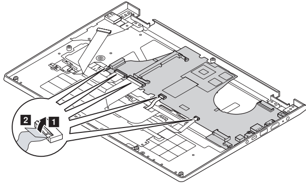
Figure 9. Removal steps of system board
