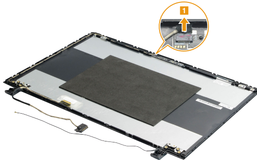
Figure 14. Removal steps of EDP cable, antenna assembly, and integrated camera
