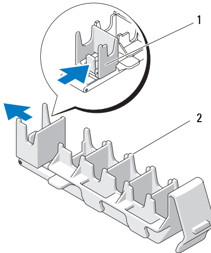
1 removable card-retention device 2 card-retention mechanism
