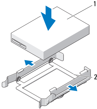
2 hard-drive bracket
