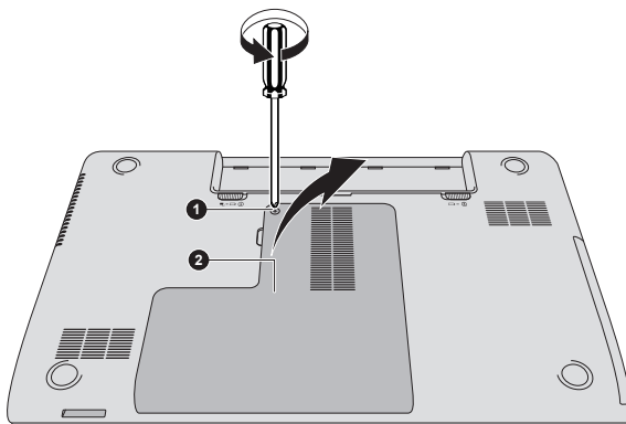
Figure 4-8 Removing the memory module cover
