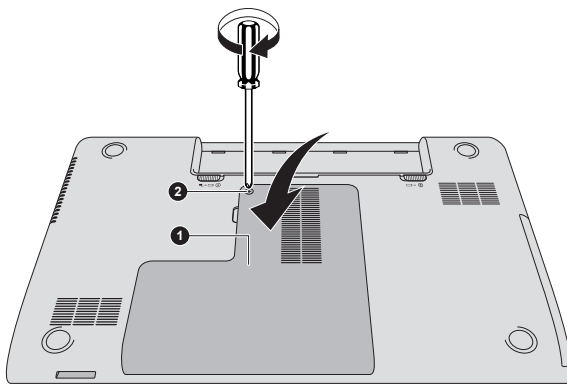
Figure 4-10 Seating the memory module cover
