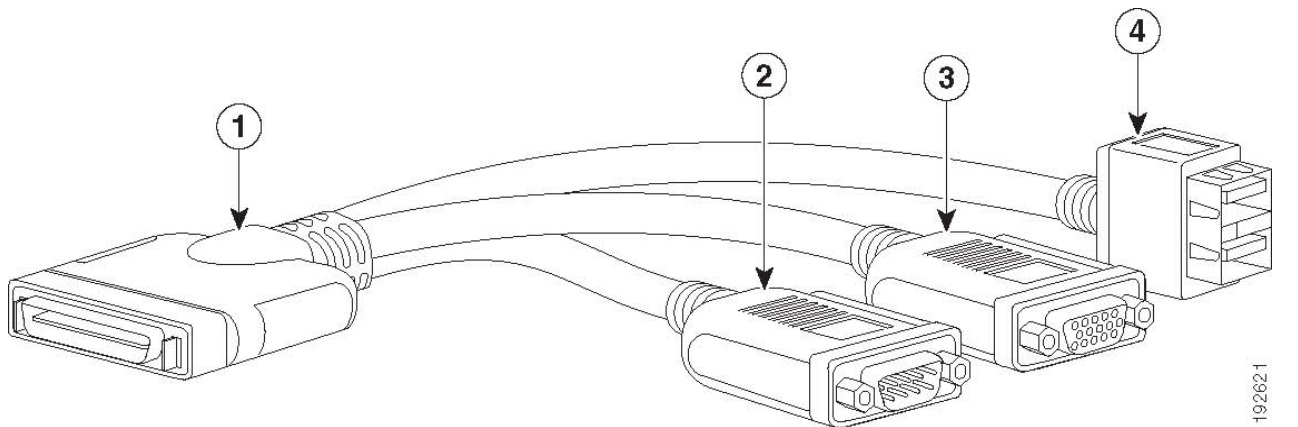
Figure 4 KVM Cable
