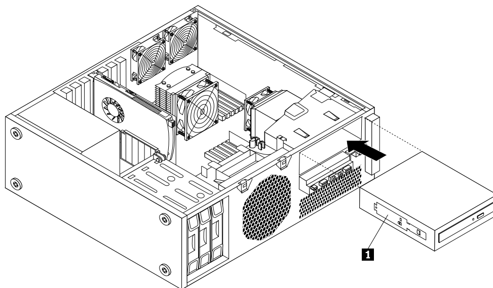
Figure 25. Installing the new optical drive
