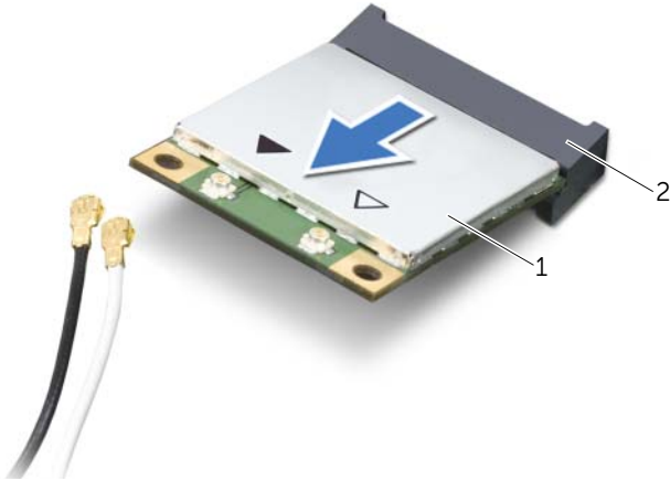
1 wireless mini-card 2 mini-card connector
