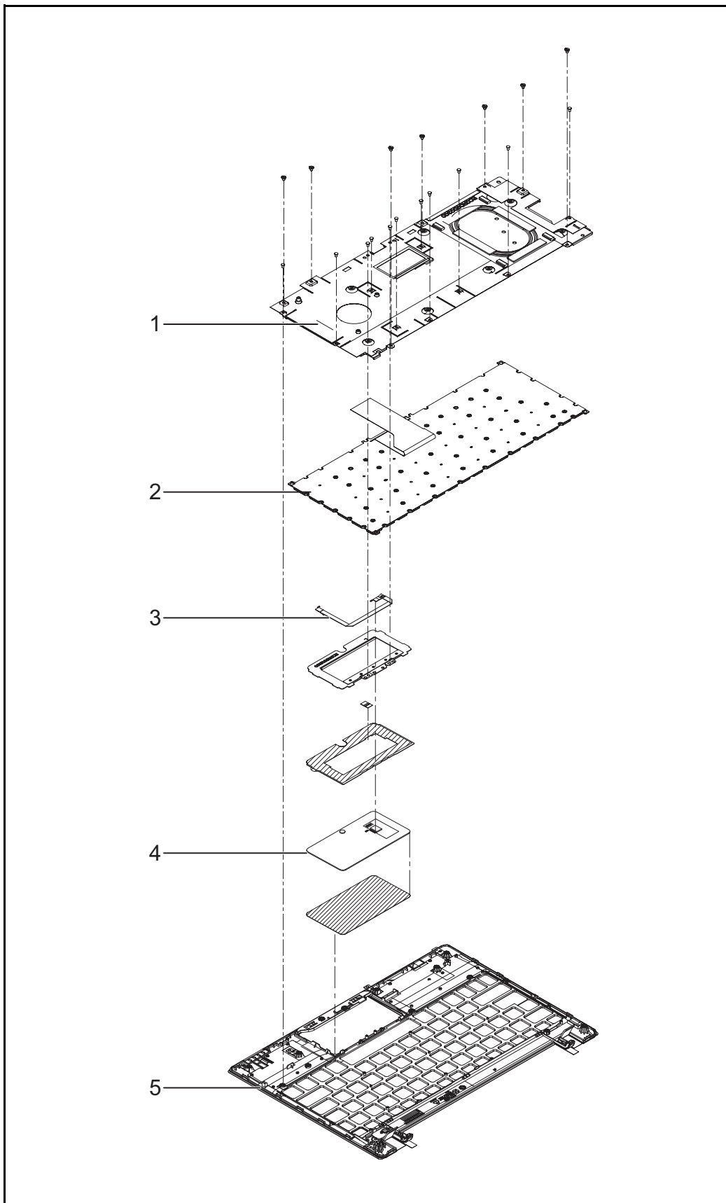
Figure 6:3. Upper Case Assembly Exploded Diagram
