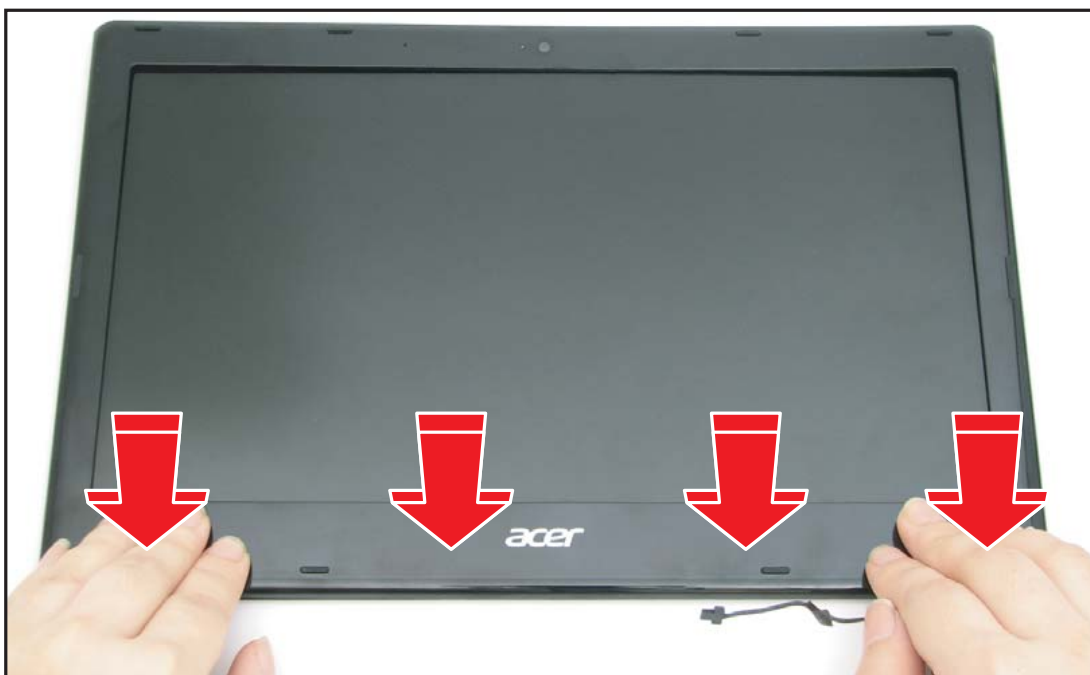
Figure 5:106. Installing the LCD Bezel (2 of 3)
