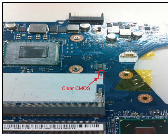
Figure 2:30. R74 Jumper
