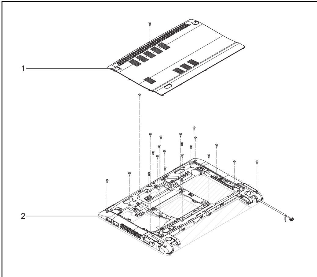
Figure 6:2. Lower Case Assembly Exploded Diagram
