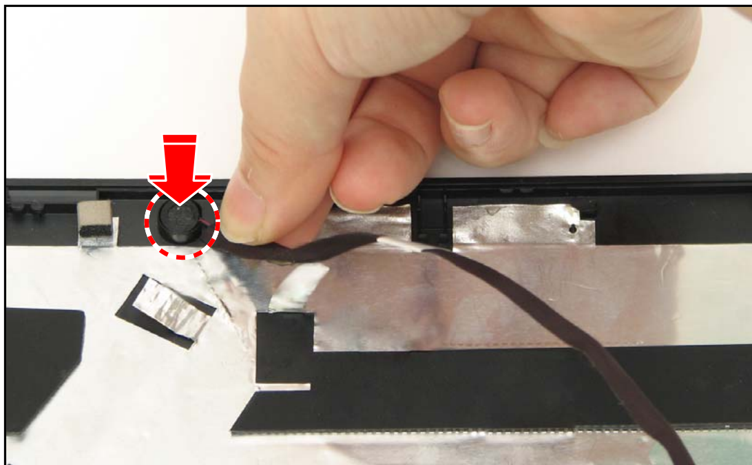
Figure 5:134. Installing the Microphone (1 of 2)
