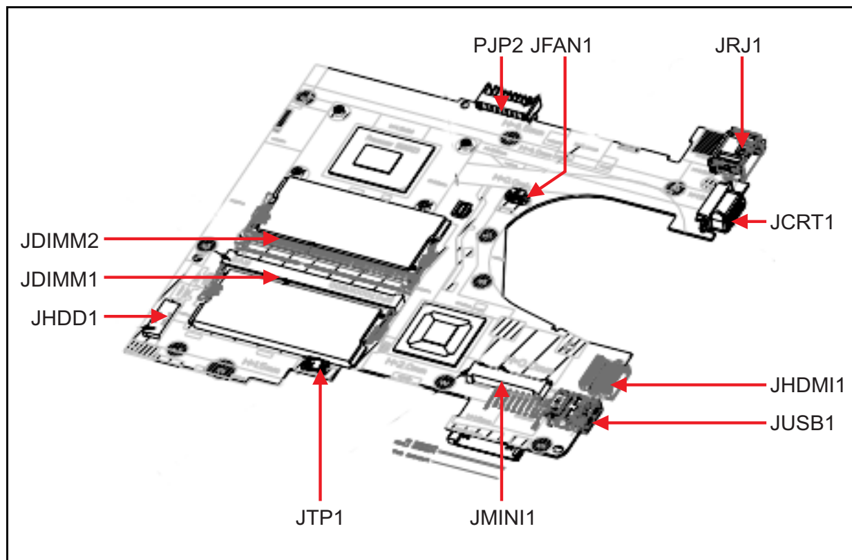
Figure 3:2. Mainboard Bottom
