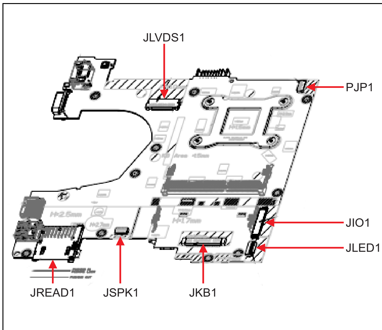
Figure 3:1. Mainboard Top
