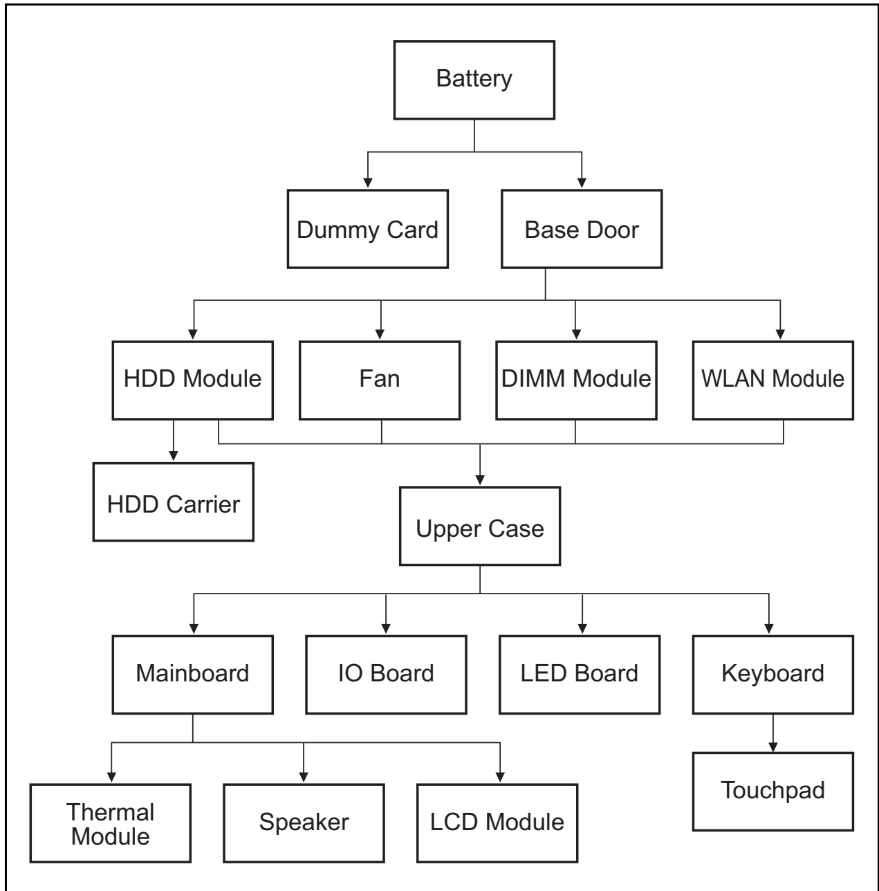
Figure 5:1. Maintenance Flow
