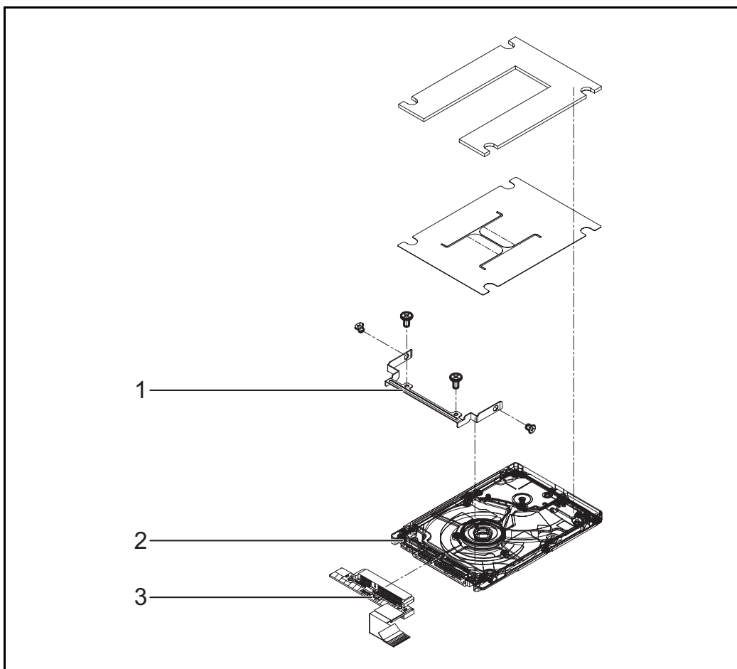
Figure 6:5. HDD Assembly Exploded Diagram
