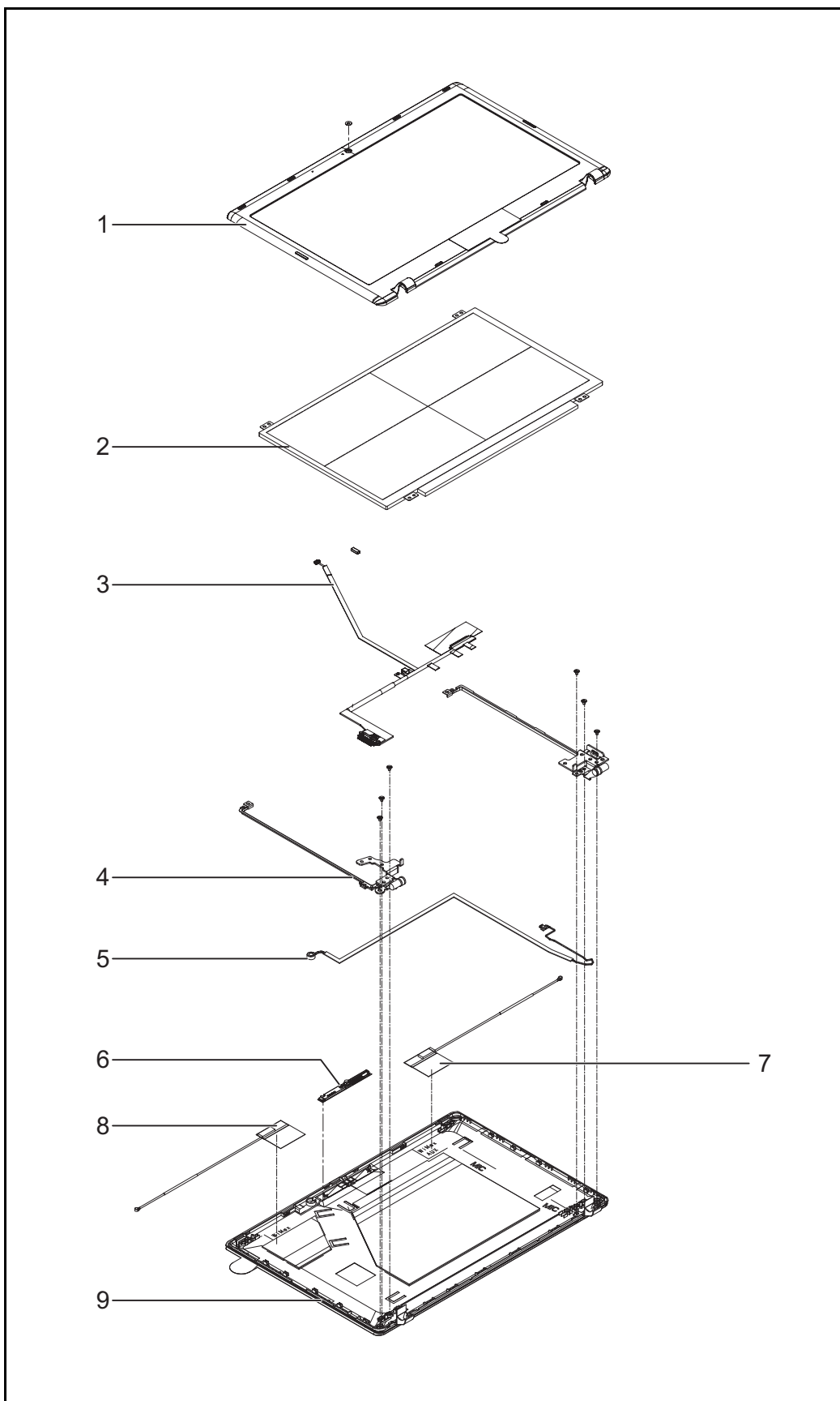
Figure 6:4. LCD Assembly Exploded Diagram
