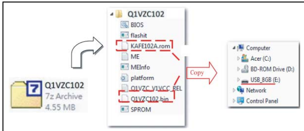
Figure 2:37. Copy *.BIN and *.ROM Files to USB Disk
