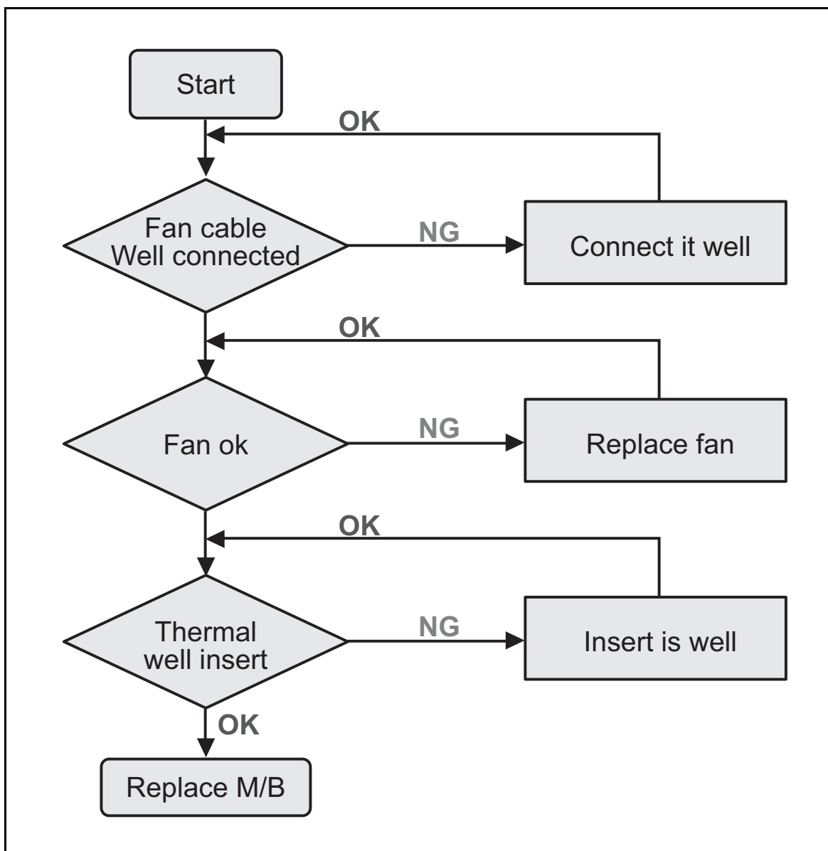
Figure 4:11. Unit Thermal Failure
