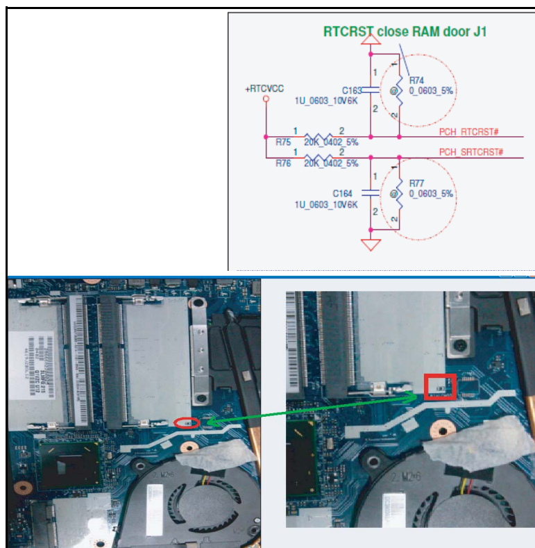
Figure 4:13. Discharge MB CMOS
