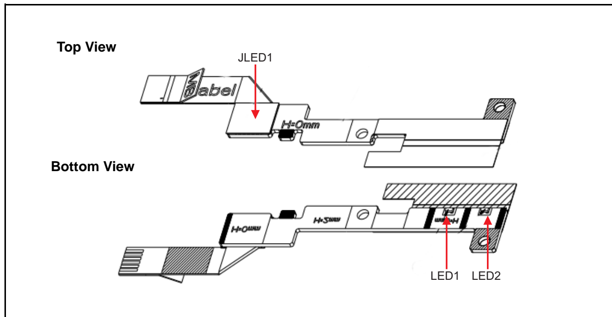
Figure 3:3. LED Board Jumper
