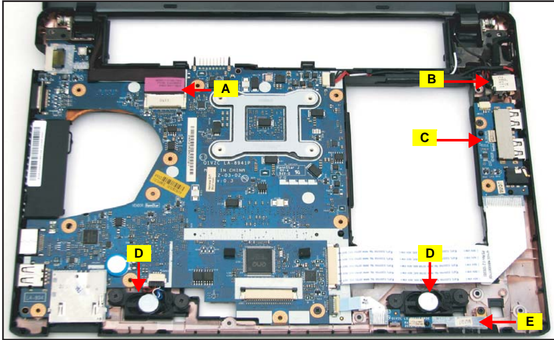
Figure 5:45. Mainboard Overview
