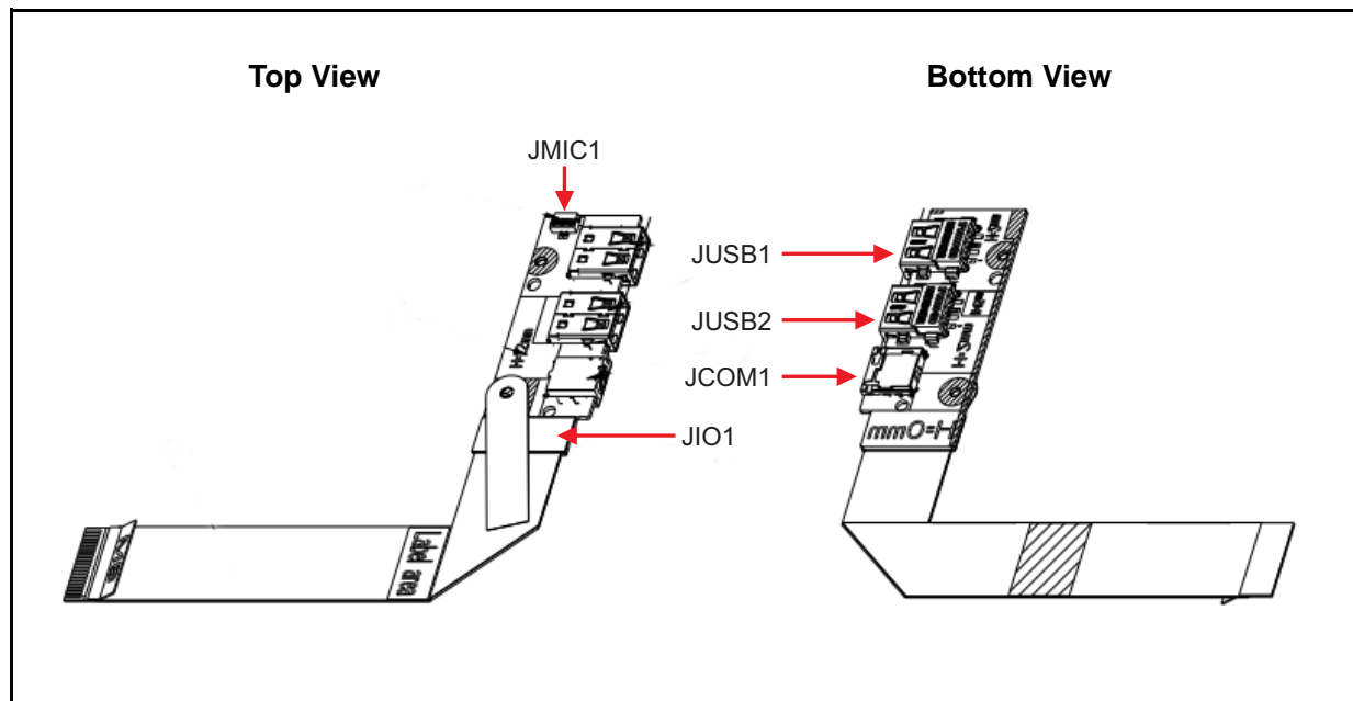
Figure 3:4. IO Board Jumper
