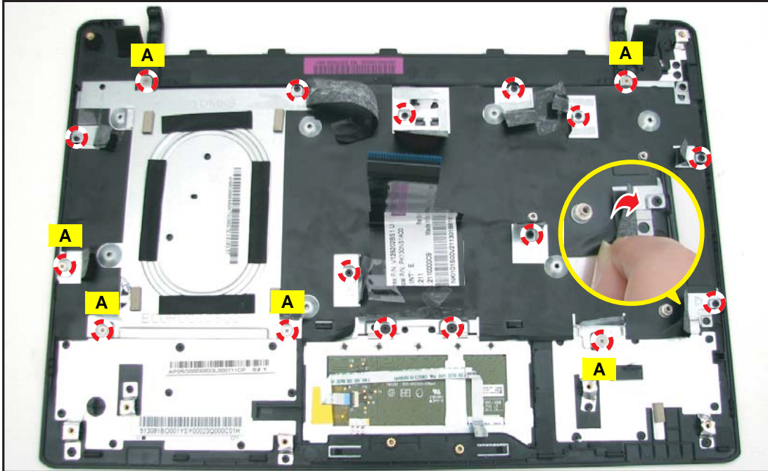
Figure 5:79. Securing the Keyboard Plastic
