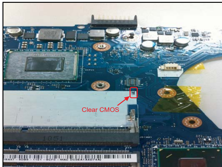
Figure 3:6. Clear CMOS
