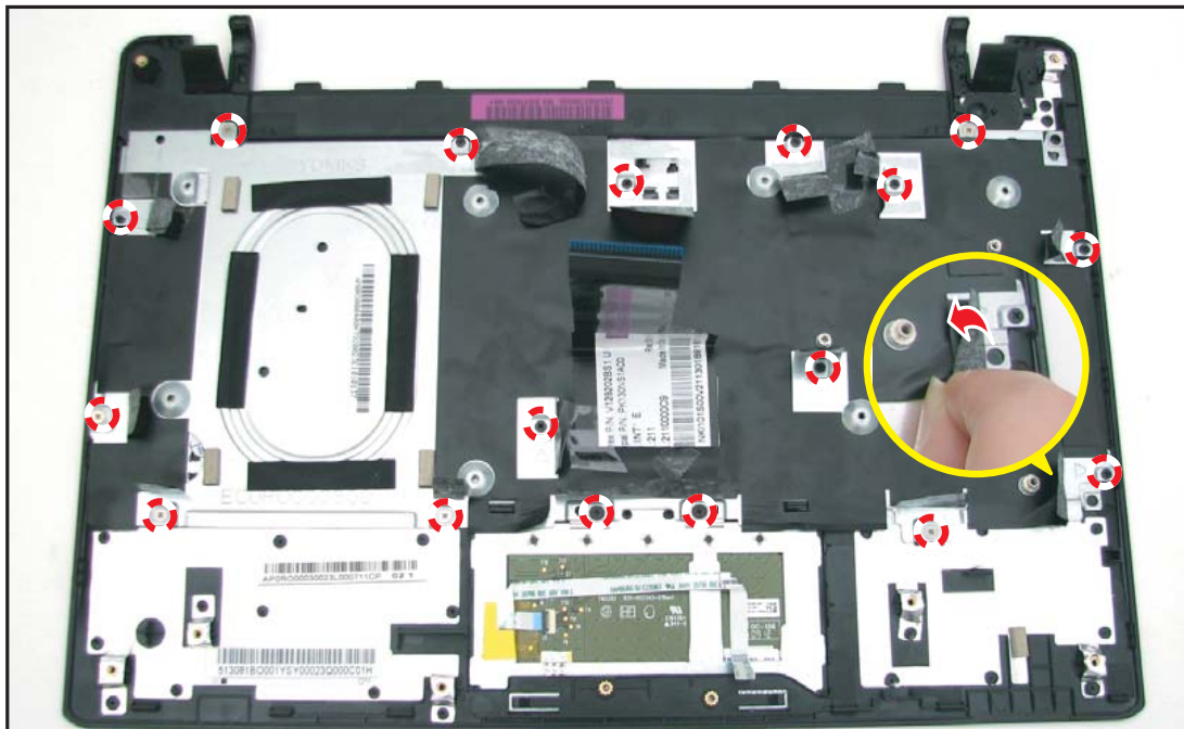
Figure 5:74. Removing the Keyboard Screws
