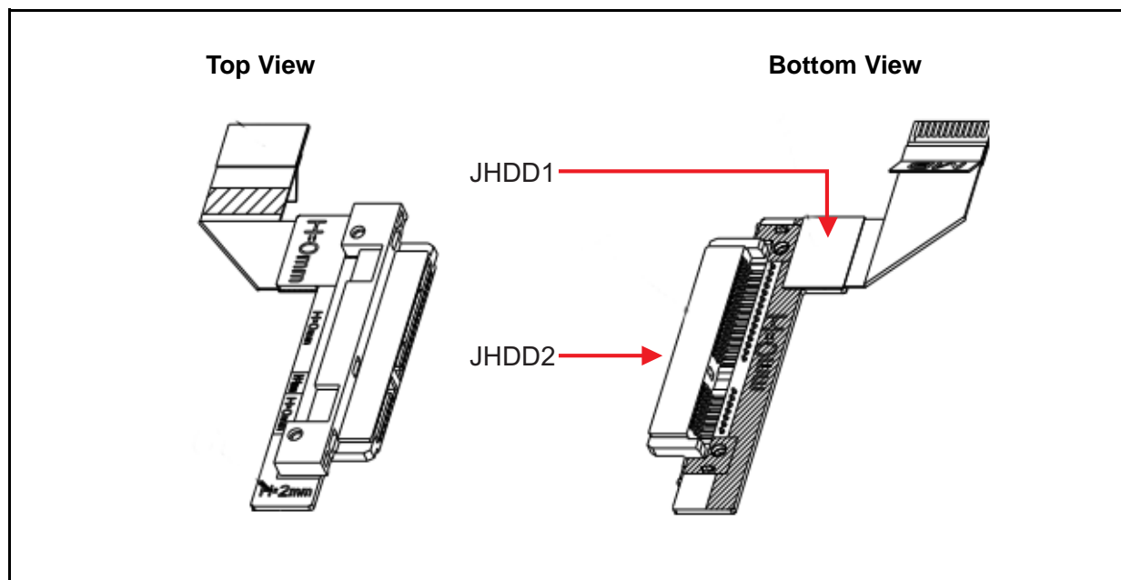
Figure 3:5. IO Board Jumper
